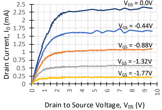
Typical Output @ V_{GS(OFF)} = -2.65
