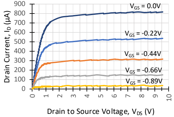
Typical Output @ V_{GS(OFF)} = -1.35
