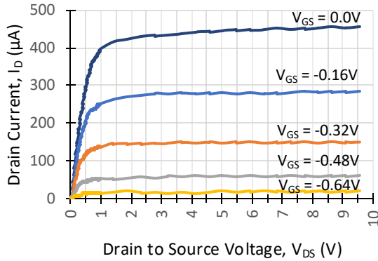
Typical Output @ V_{GS(OFF)} = -0.96
