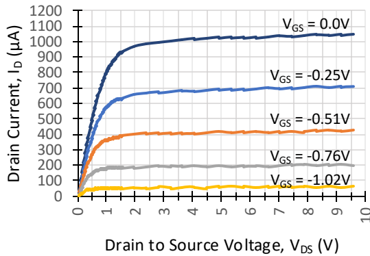
Typical Output @ V_{GS(OFF)} = -1.5
