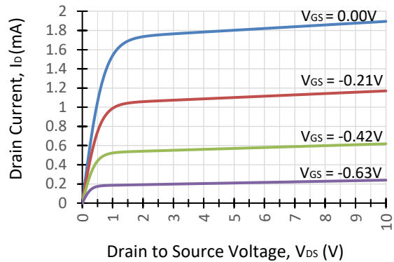
Typical Output given V_{GS(OFF)}
