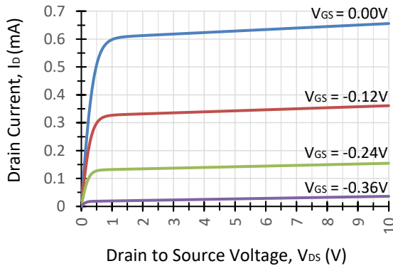
Typical Output @ V_{GS(OFF)} = -1.17V
